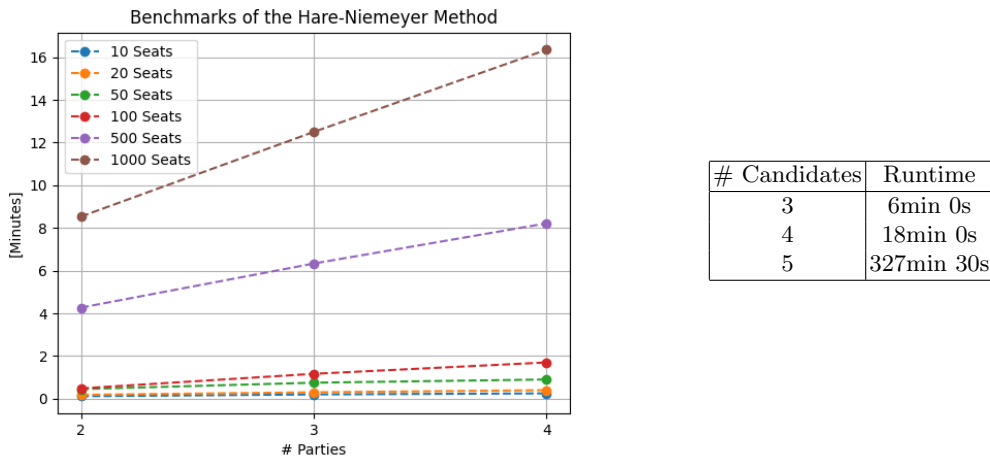
Fig. 3: Benchmarks for the Hare-Niemeyer method (left) and IRV (right).
