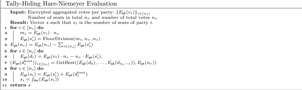
Fig. 2: Tally-Hiding Hare-Niemeyer Evaluation
